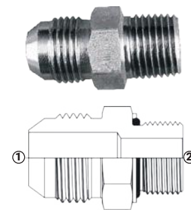
(1) Macho JIC (2) Macho BSPT
