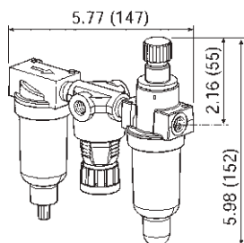
1.60 (41) Bowl Removal Clearance
