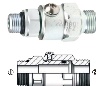
(1) Macho ORB (2) Macho Face Seal
