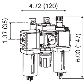
1.31 (33) Bowl Removal Clearance
