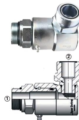
(1) Macho ORB (2) Macho FS
